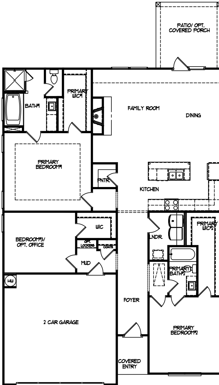
Main Level
